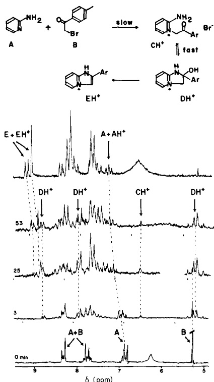
Fig. 1. Partial 100 MHz ^1\text{H} NMR spectra of a DMSO- d_6 solution recorded 3, 25, and 53 minutes after mixing 2-aminopyridine and p -methylphenacyl bromide. The bottom scan is the sum of separately recorded spectra of the two starting materials. The top scan was recorded after no further changes occurred (18 hr). The two lowest spectra are attenuated. Chemical shifts refer to all scans and are relative to external TMS. Relevant assignments are as follows: bottom scan: 5.25 (s): \text{CH}_2 protons; 6.9 (m): overlapping H-3 and H-5 signals; 8.3 (m): overlapping signals of ortho -protons of B and H-6 of A; signals connected by dotted lines: A + \text{AH}^+ (t): H-5 of protonated and non-protonated species; \text{CH}^+ (s): \text{CH}_2 protons; \text{DH}^+ : 5.2(q), \text{CH}_2 protons; 7.95 (d), phenyl protons ortho to carbinolamine substituent; 8.8 (d), proton \alpha to pyridinium nitrogen; E + \text{EH}^+ : H-3 (s) and H-5 (d) of protonated and nonprotonated species. Top scan: broad peak: NH and \text{H}_2\text{O} protons; 5.2 (s), side product (see Ref. 10).
